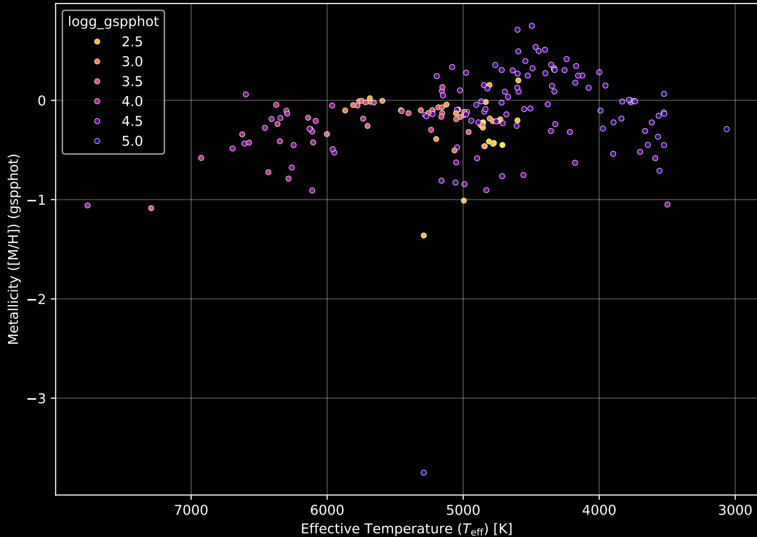
APOGEE DR17 Field: [170+60] Stellar Population Parameters (n= 186)
