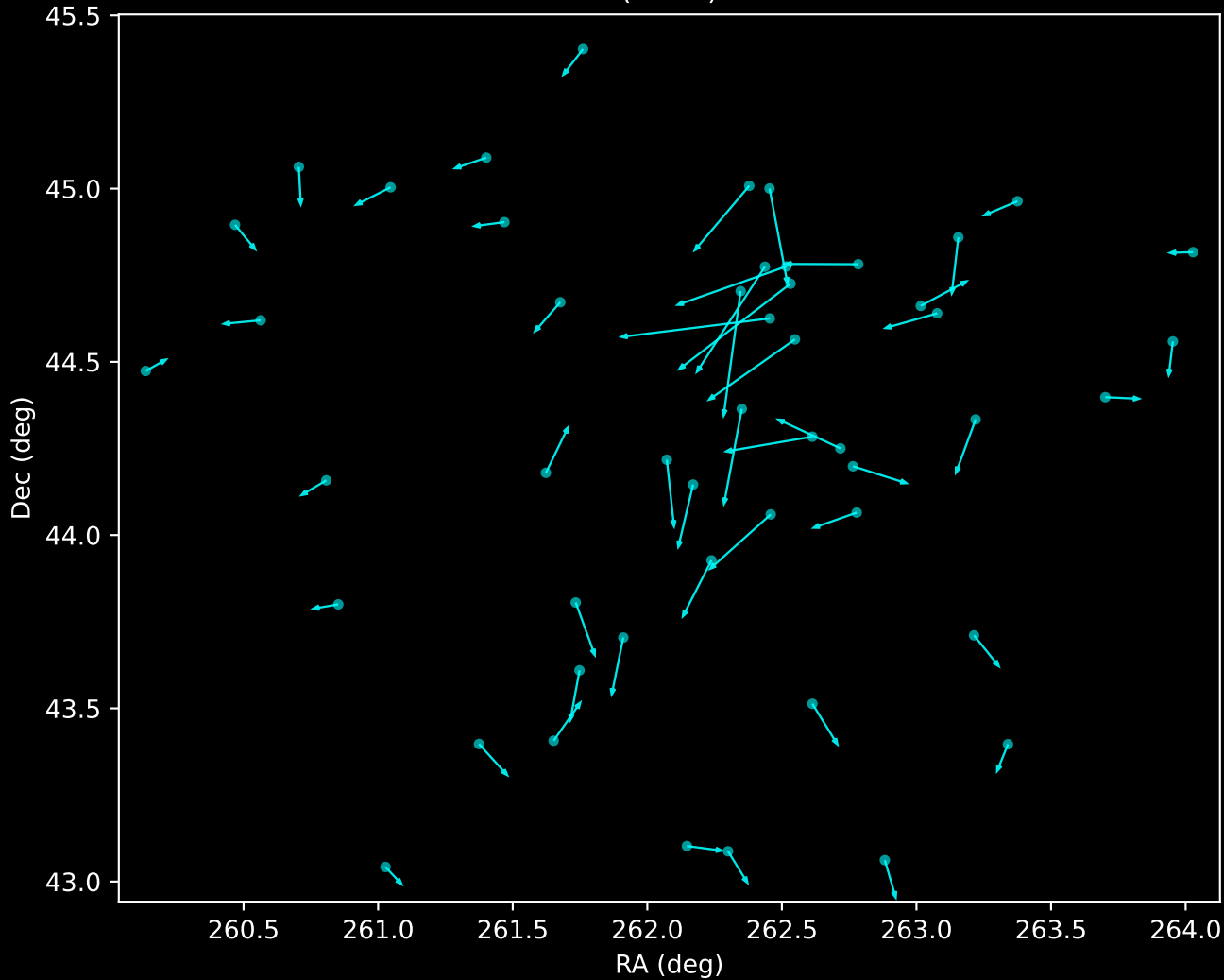
APOGEE DR17 Noise Stream Proper Motion Vectors (n=50)
