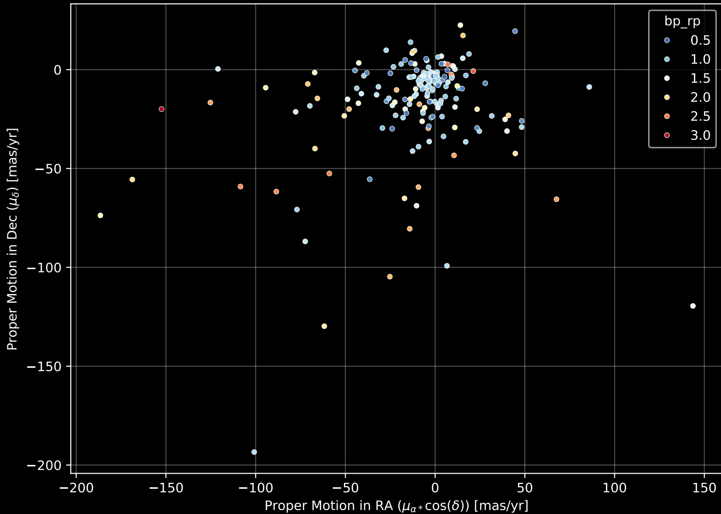
APOGEE DR17 Field: [170+60] Proper Motion Diagram (n= 186)
