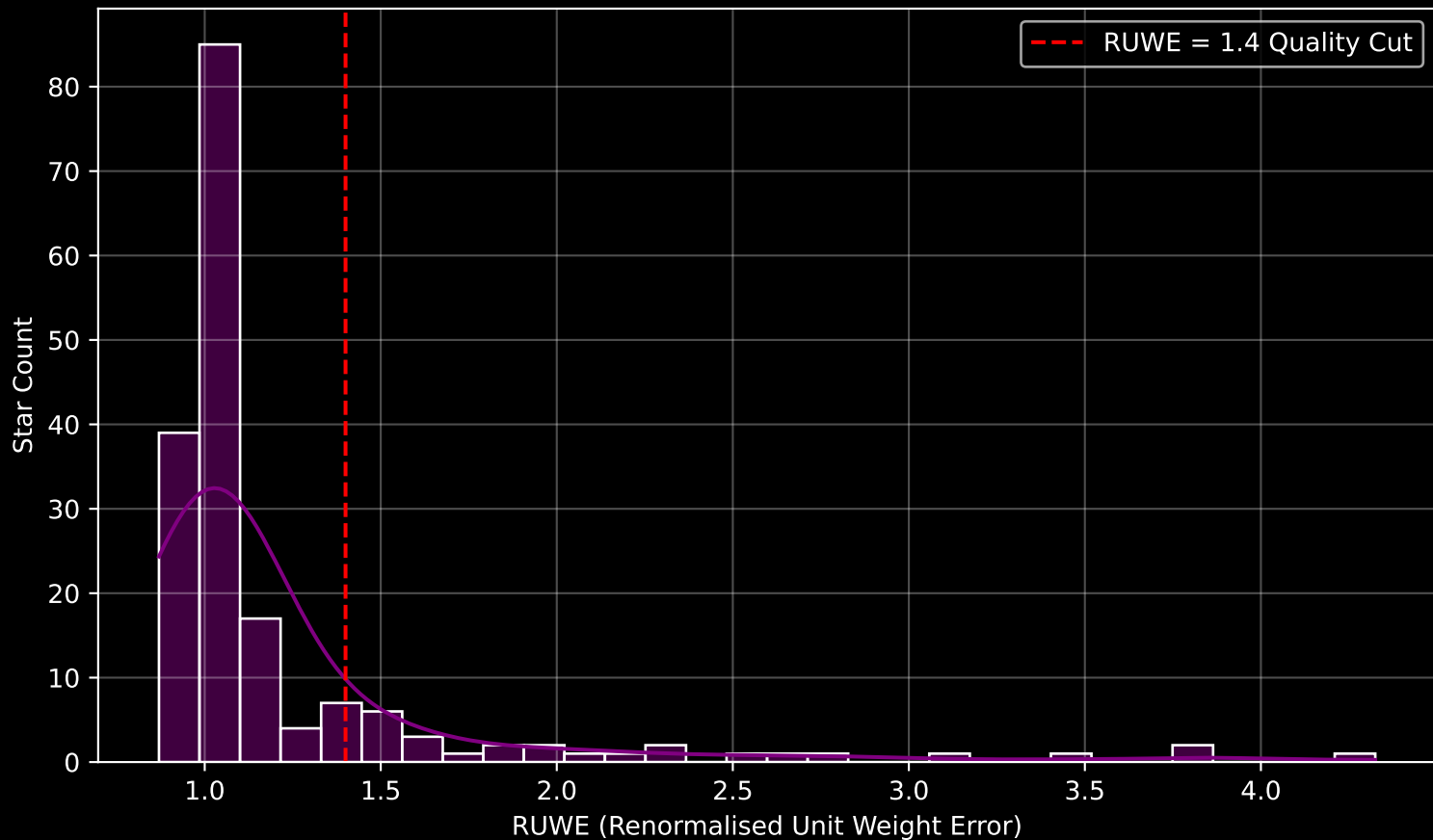
GAPOGEE DR17 Field [170+60] RUWE Distribution (n= 178)
