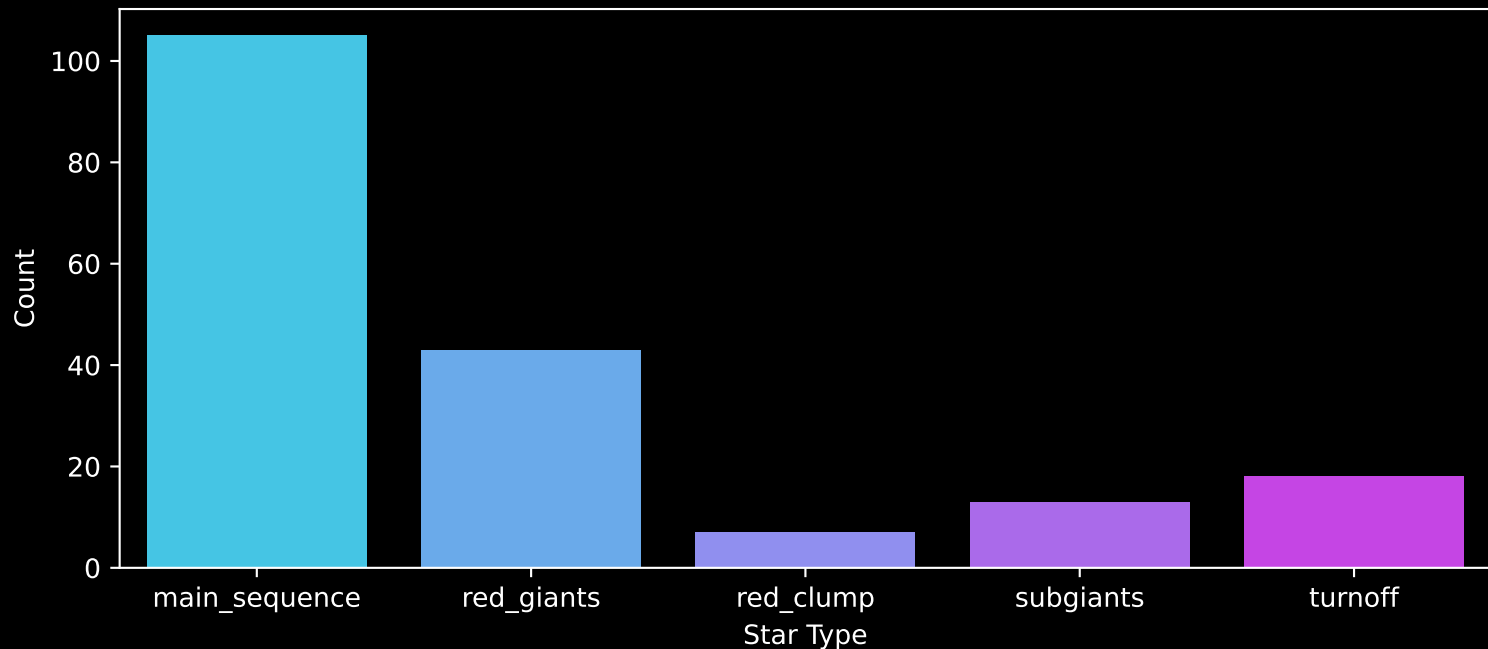
APOGEE DR17 Field: [170+60] Count plot of Star Type
