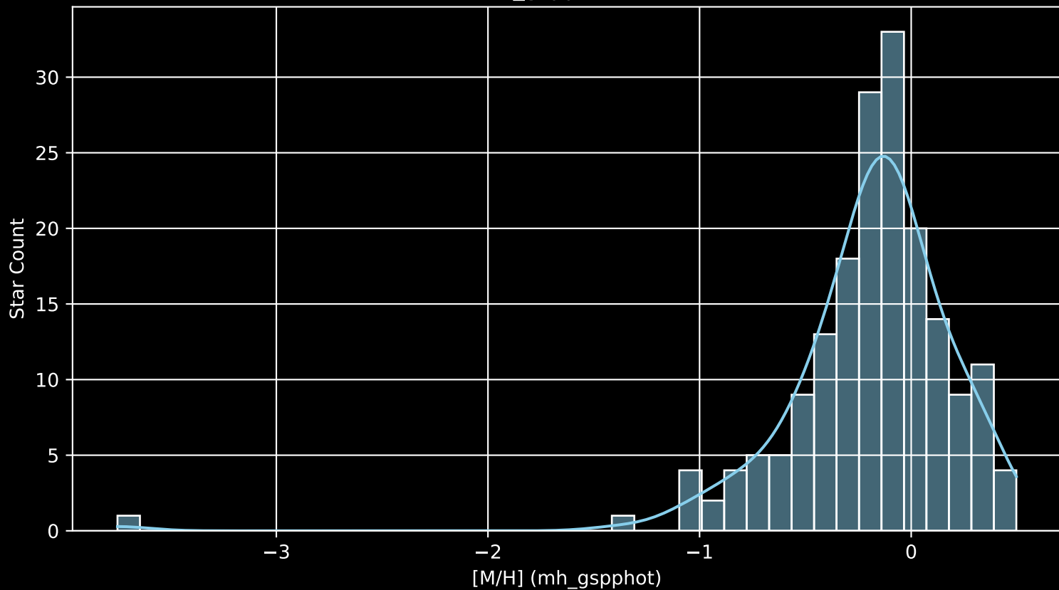
APOGEE DR17 Field: [170+60 [M/H] (mh_gspphot) (n= 182)
