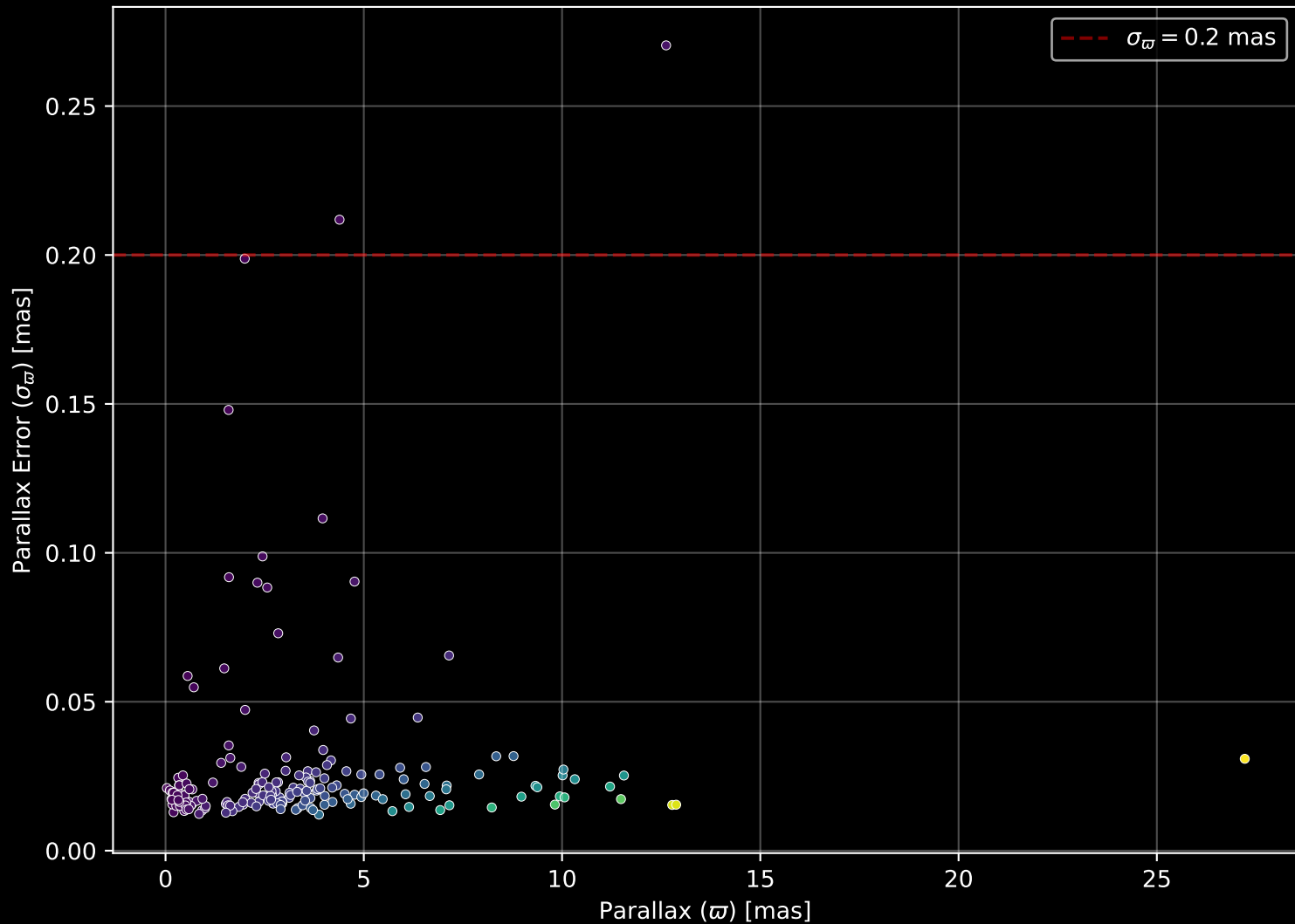
APOGEE DR17 Field: [170+60] Parallax Quality (n= 186)
